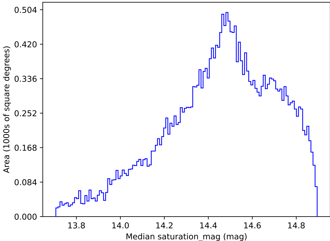
too_elab_r16_d3_griz_v3.4_10yrs All sky i band: Median saturation_mag
