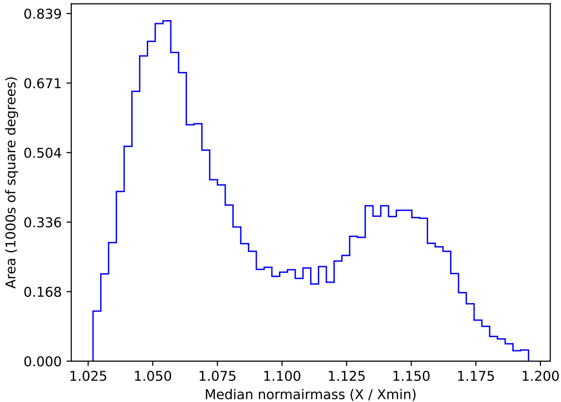
too_elab_r16_d3_griz_v3.4_10yrs WFD y band: Median normairmass
