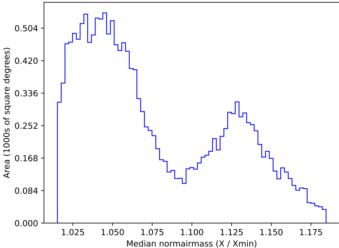
too_elab_r16_d3_griz_v3.4_10yrs WFD r band: Median normairmass
