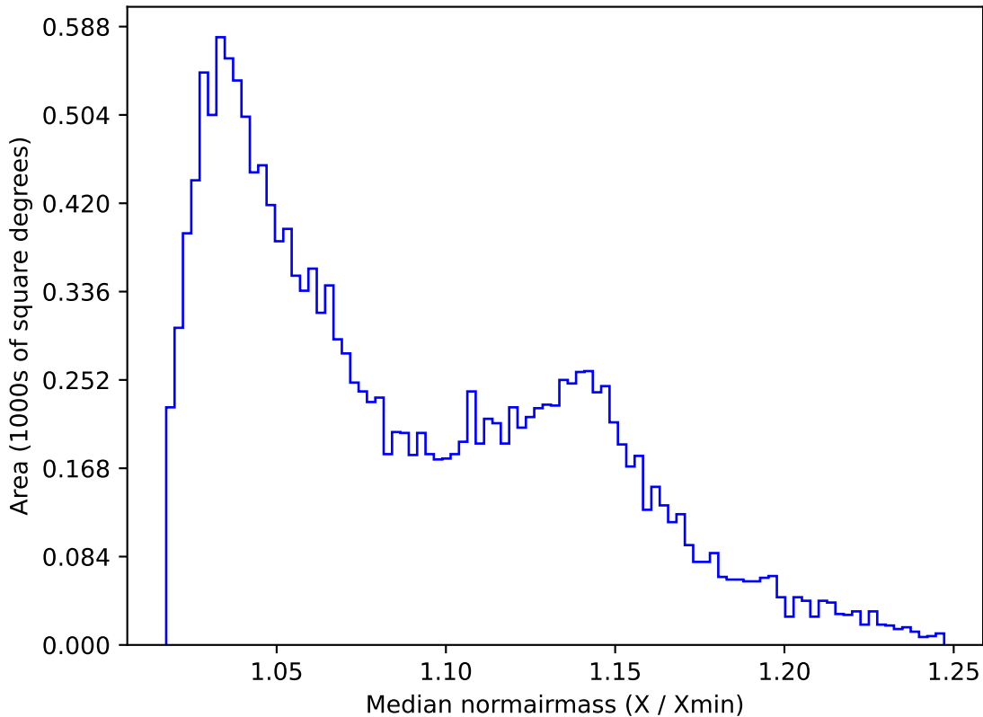
too_elab_r16_d3_griz_v3.4_10yrs WFD g band: Median normairmass
