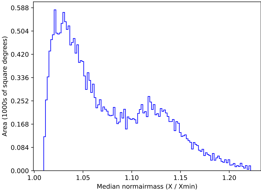
too_elab_r16_d3_griz_v3.4_10yrs All sky u band: Median normairmass
