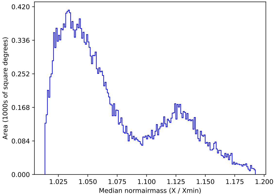
too_elab_r16_d3_griz_v3.4_10yrs All sky r band: Median normairmass
