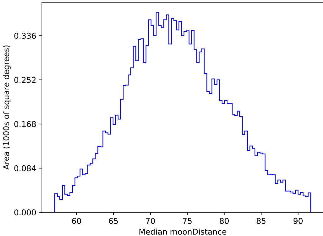
too_elab_r16_d3_griz_v3.4_10yrs WFD z band: Median moonDistance
