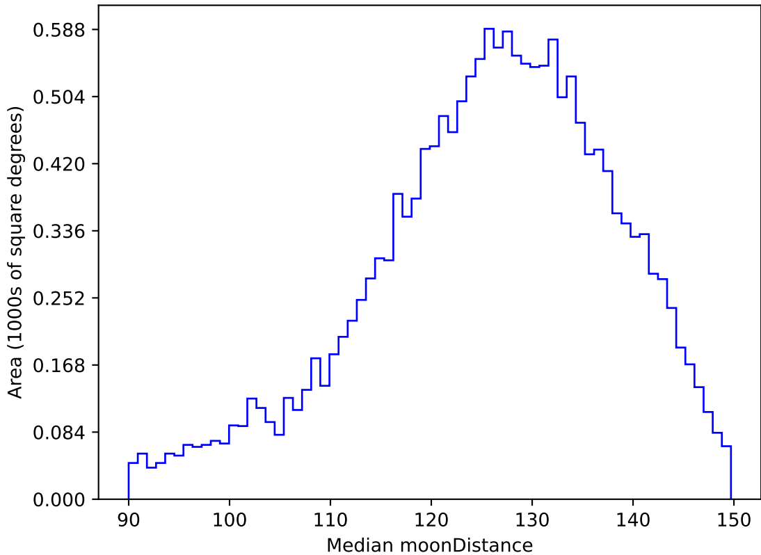
too_elab_r16_d3_griz_v3.4_10yrs WFD u band: Median moonDistance
