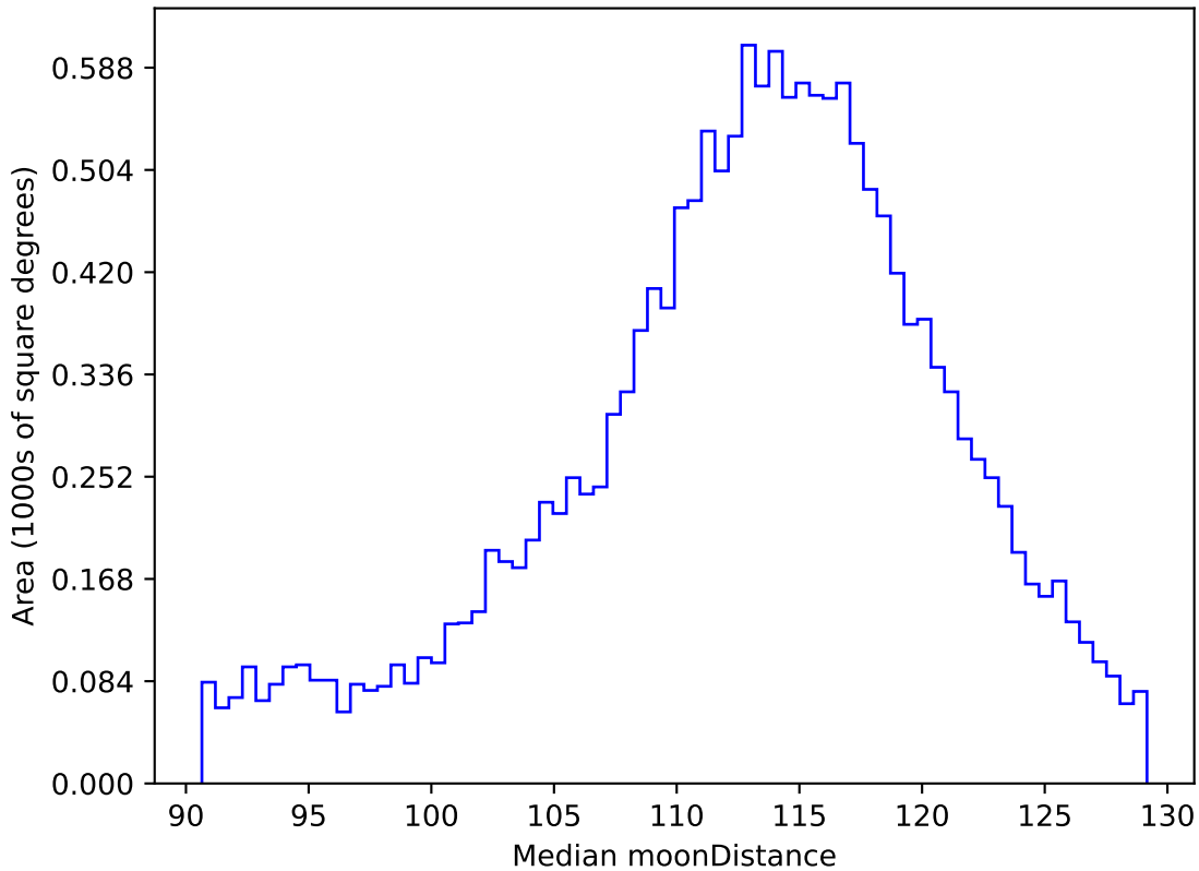
too_elab_r16_d3_griz_v3.4_10yrs WFD r band: Median moonDistance
