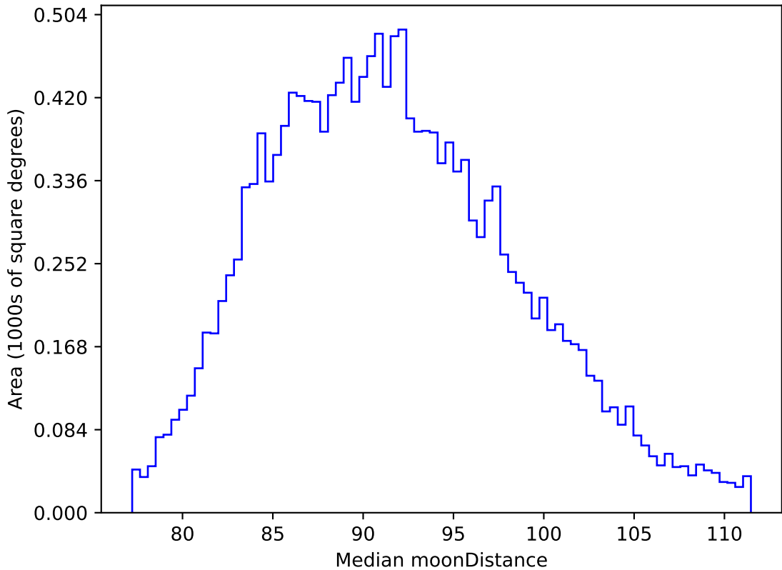
too_elab_r16_d3_griz_v3.4_10yrs WFD i band: Median moonDistance
