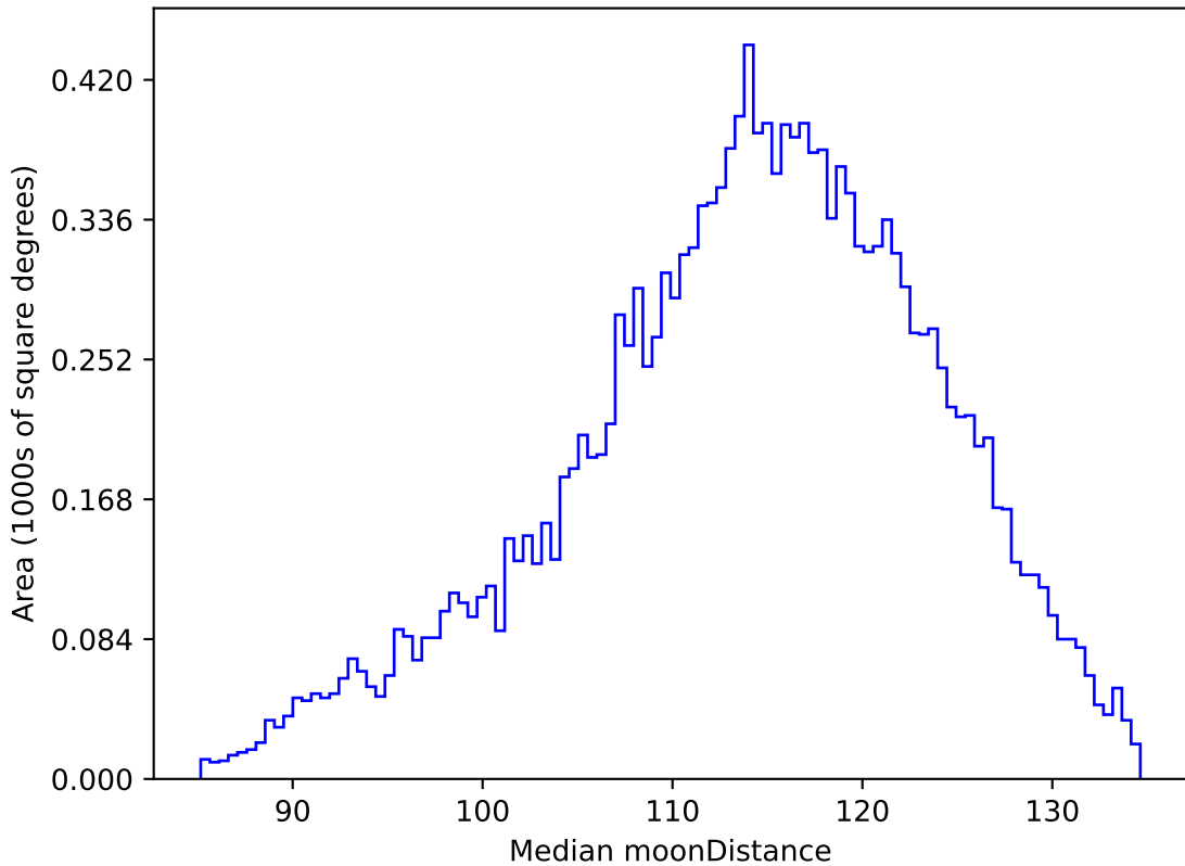
too_elab_r16_d3_griz_v3.4_10yrs WFD g band: Median moonDistance
