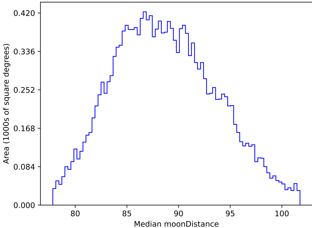
too_elab_r16_d3_griz_v3.4_10yrs WFD all bands: Median moonDistance
