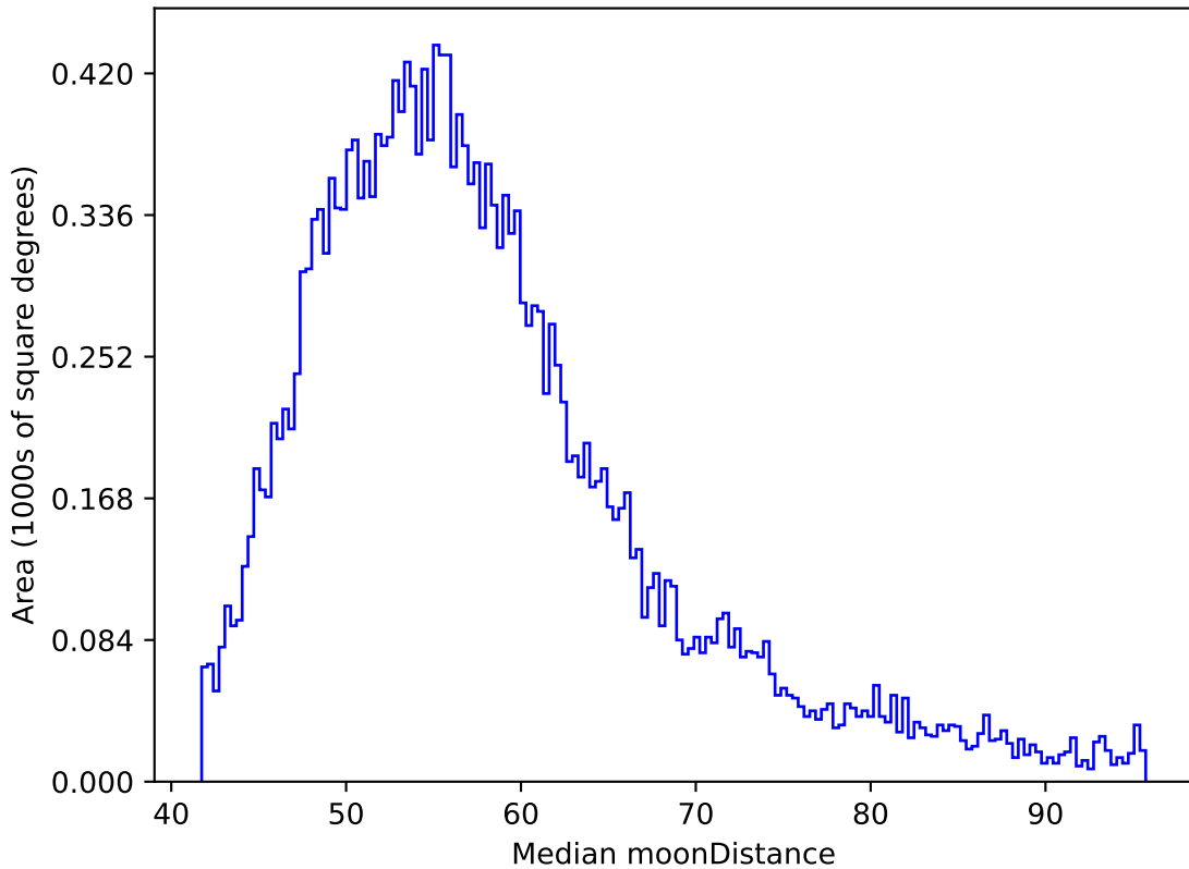
too_elab_r16_d3_griz_v3.4_10yrs All sky y band: Median moonDistance
