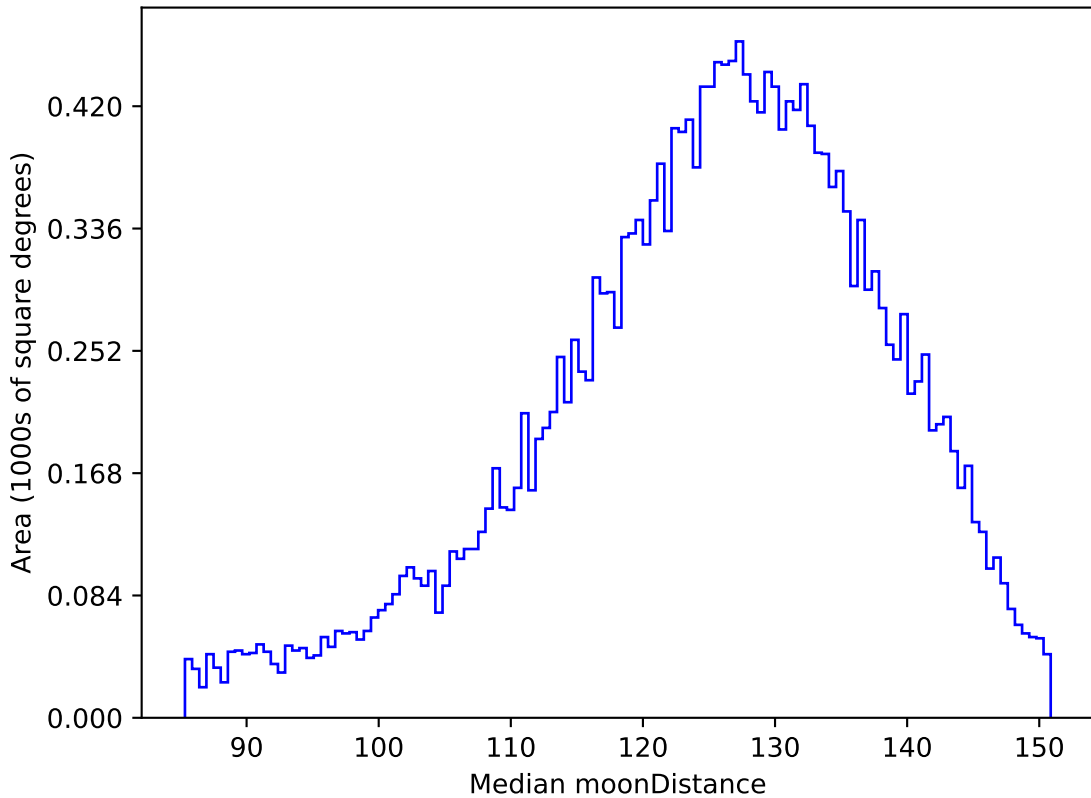
too_elab_r16_d3_griz_v3.4_10yrs All sky u band: Median moonDistance
