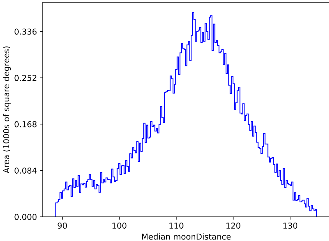
too_elab_r16_d3_griz_v3.4_10yrs All sky r band: Median moonDistance
