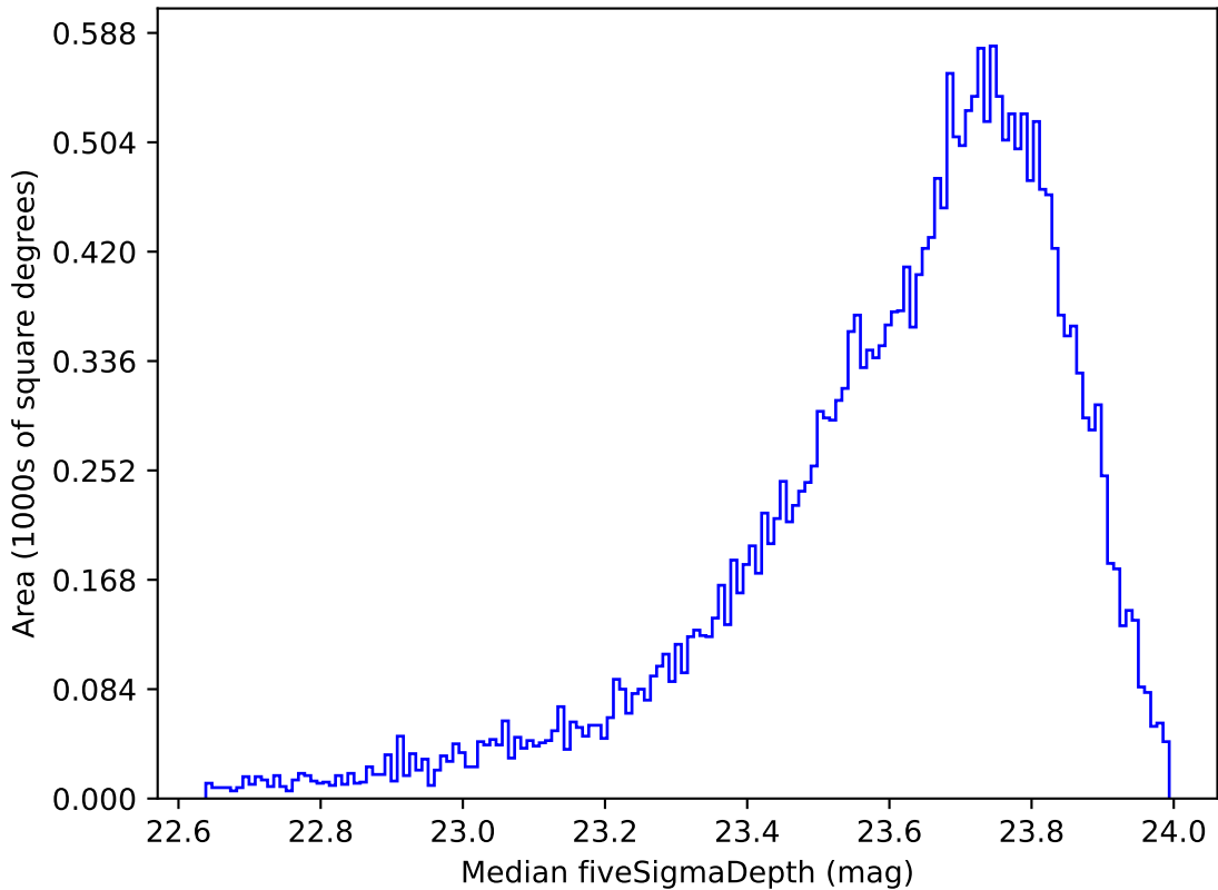
too_elab_r16_d3_griz_v3.4_10yrs Yr 1 i band: Median fiveSigmaDepth
