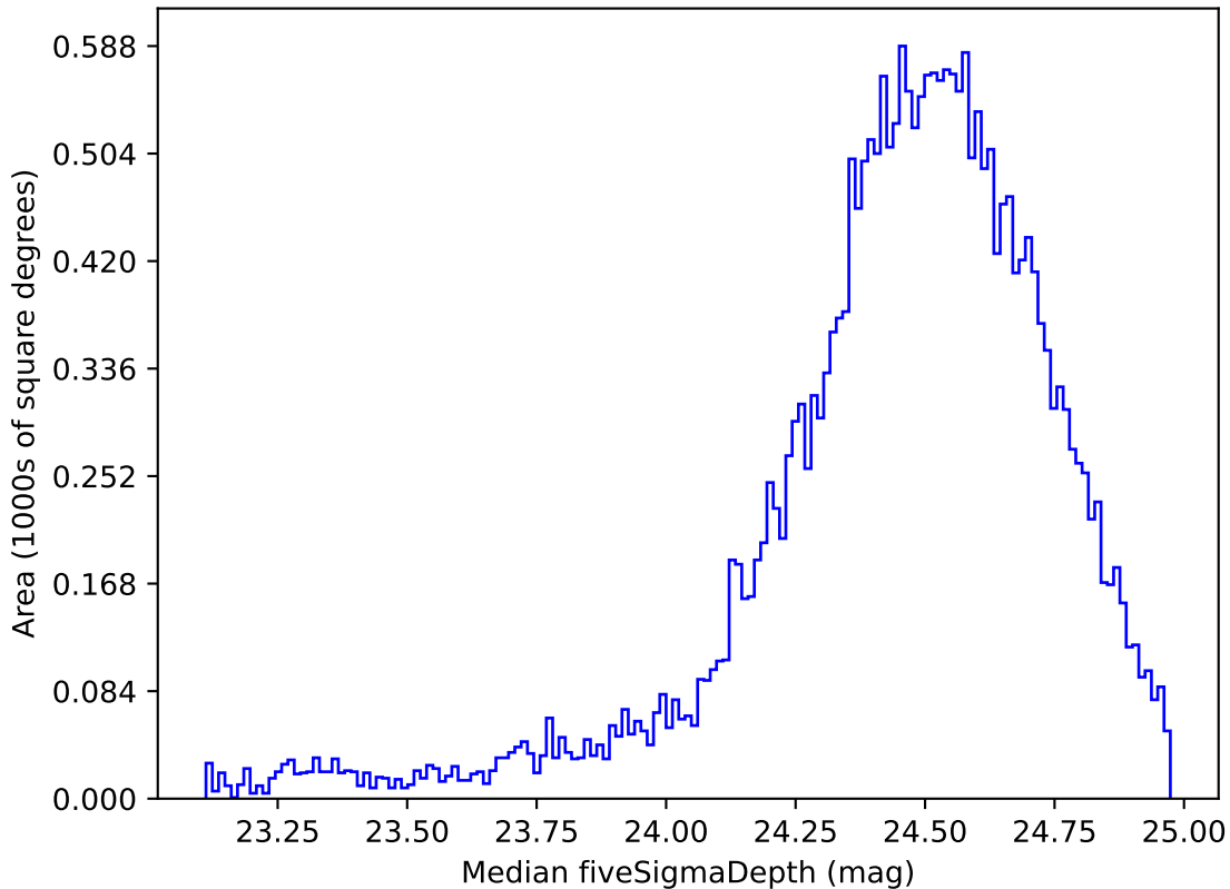
too_elab_r16_d3_griz_v3.4_10yrs Yr 1 g band: Median fiveSigmaDepth
