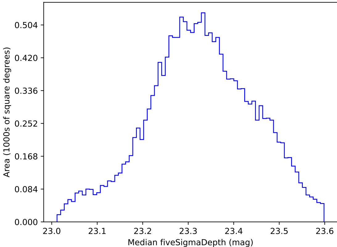
too_elab_r16_d3_griz_v3.4_10yrs WFD all bands: Median fiveSigmaDepth
