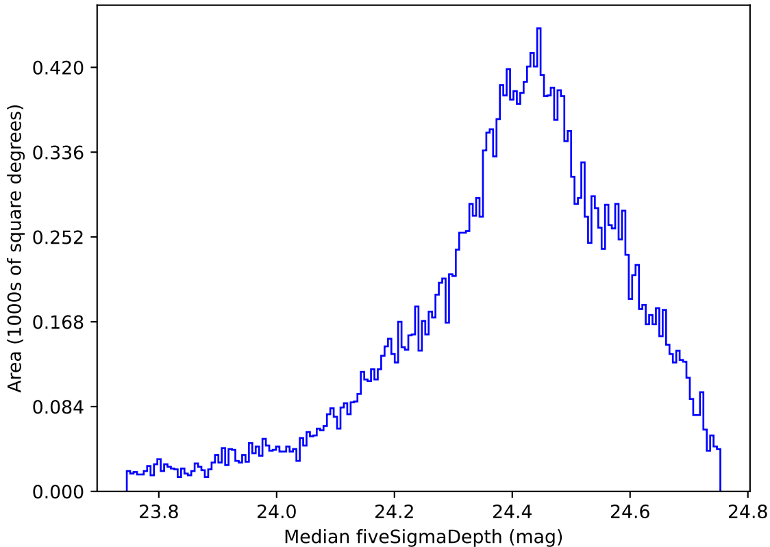
too_elab_r16_d3_griz_v3.4_10yrs All sky g band: Median fiveSigmaDepth
