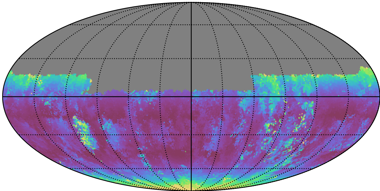
too_elab_r16_d3_griz_v3.4_10yrs Yr 1 u band: Median airmass
