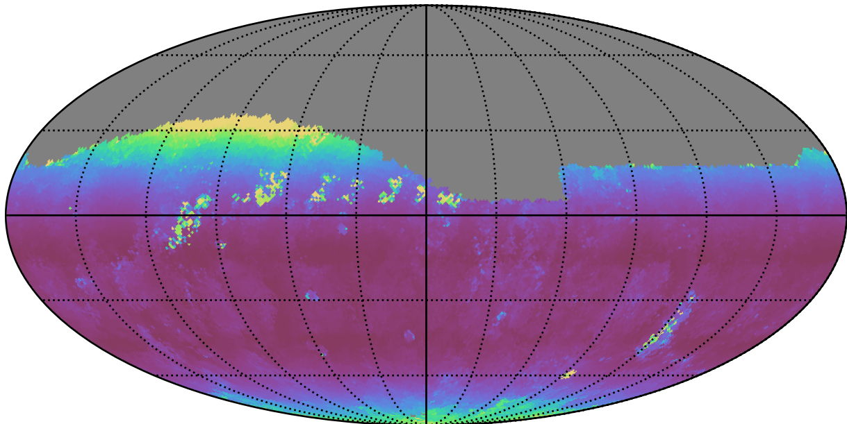
too_elab_r16_d3_griz_v3.4_10yrs Yr 1 r band: Median airmass
