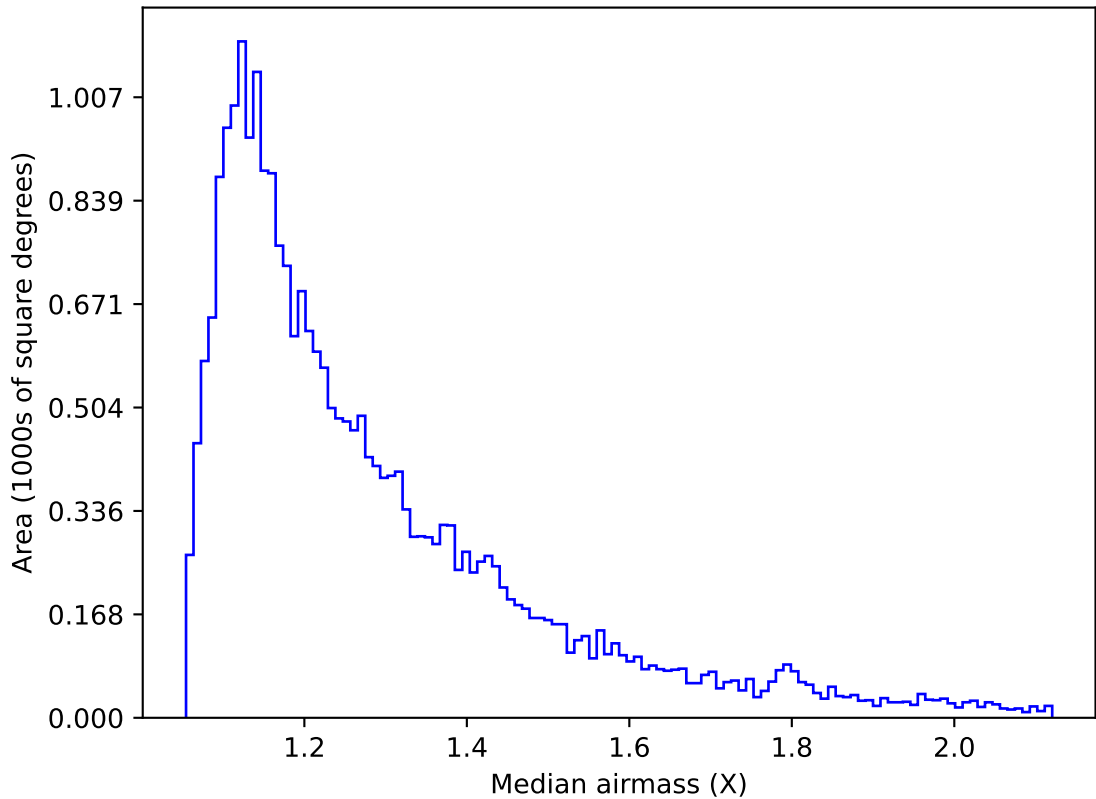
too_elab_r16_d3_griz_v3.4_10yrs Yr 1 g band: Median airmass
