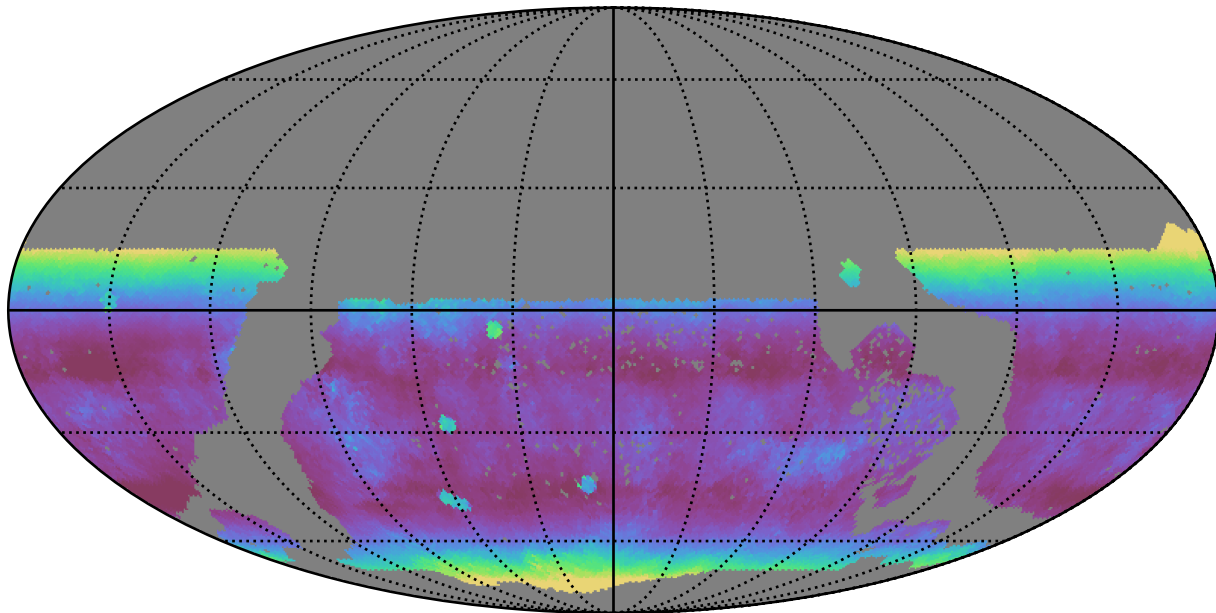
too_elab_r16_d3_griz_v3.4_10yrs WFD z band: Median airmass
