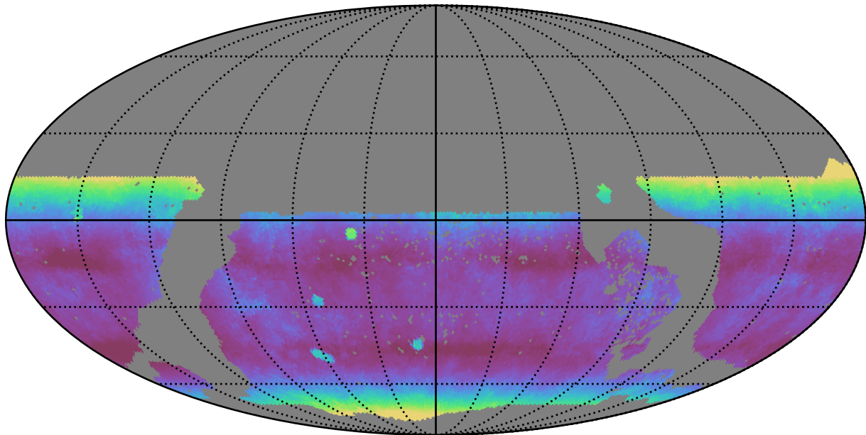
too_elab_r16_d3_griz_v3.4_10yrs WFD y band: Median airmass
