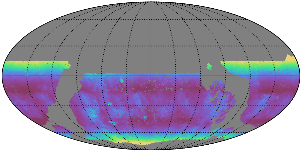
too_elab_r16_d3_griz_v3.4_10yrs WFD u band: Median airmass
