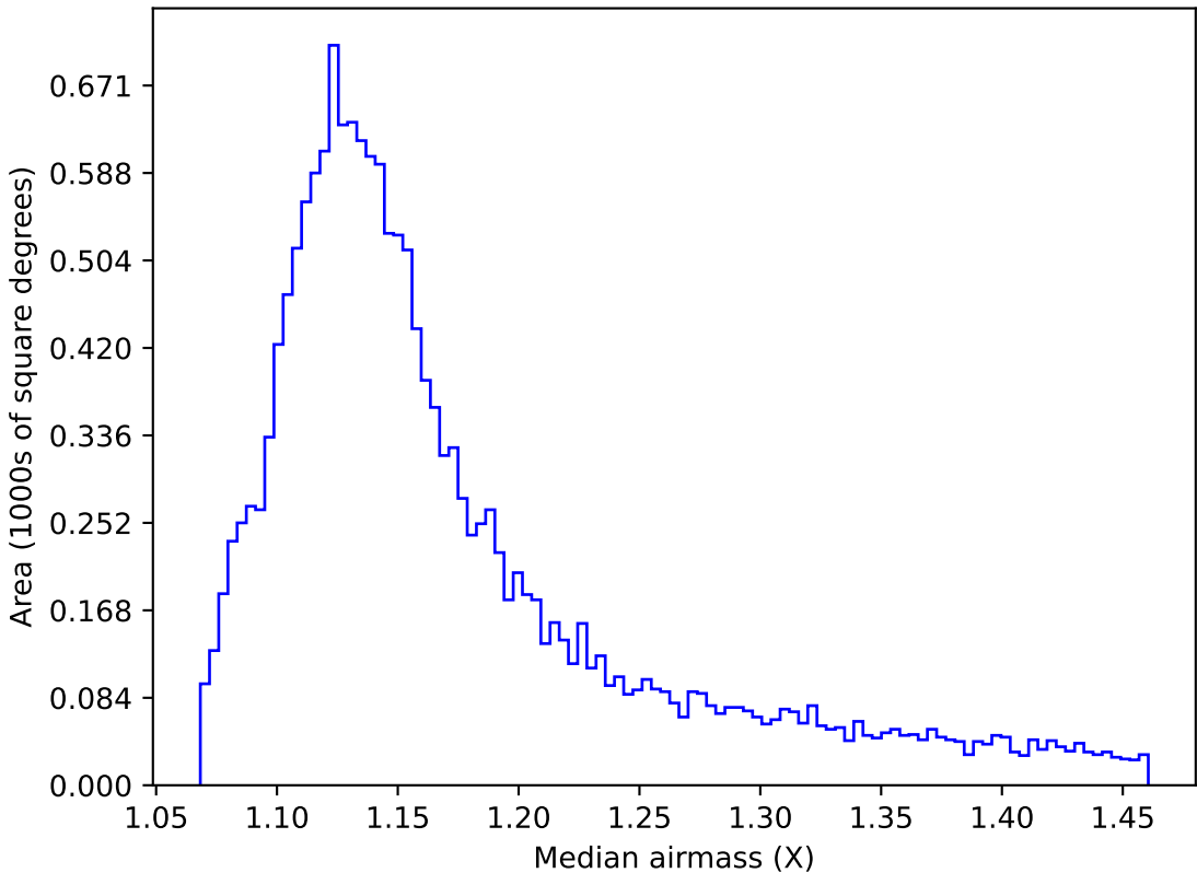
too_elab_r16_d3_griz_v3.4_10yrs WFD u band: Median airmass
