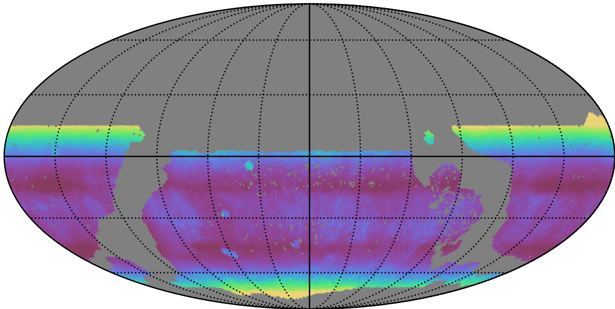
too_elab_r16_d3_griz_v3.4_10yrs WFD i band: Median airmass
