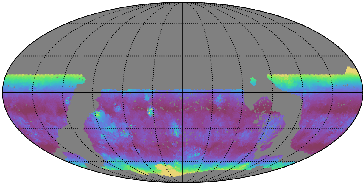
too_elab_r16_d3_griz_v3.4_10yrs WFD g band: Median airmass
