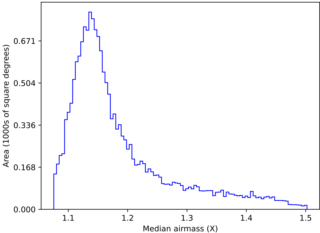
too_elab_r16_d3_griz_v3.4_10yrs WFD g band: Median airmass
