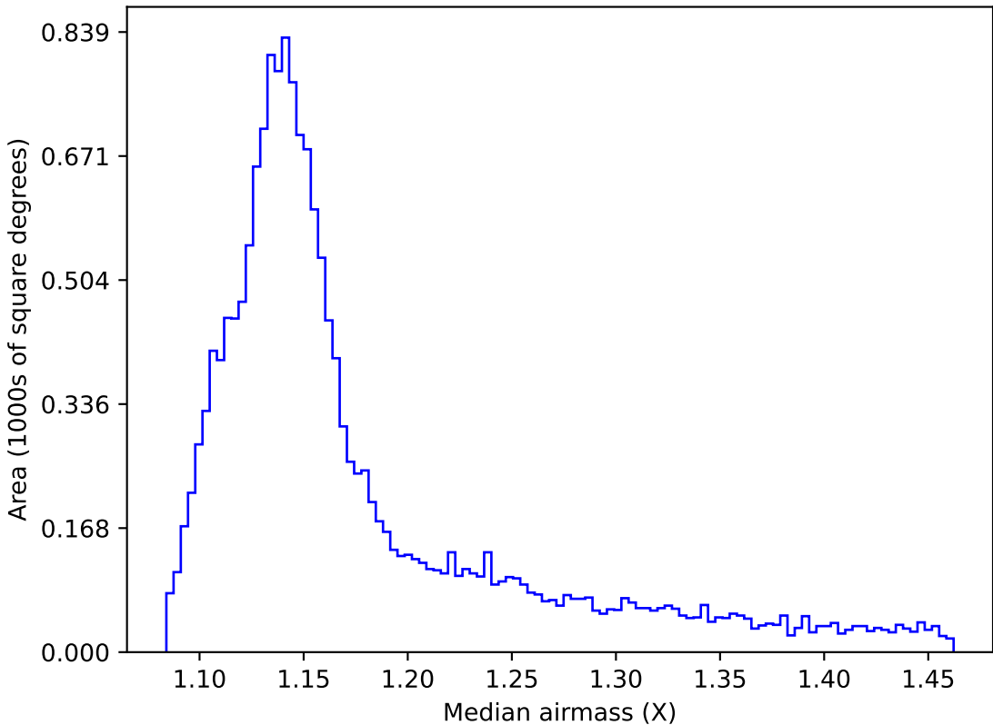
too_elab_r16_d3_griz_v3.4_10yrs WFD all bands: Median airmass
