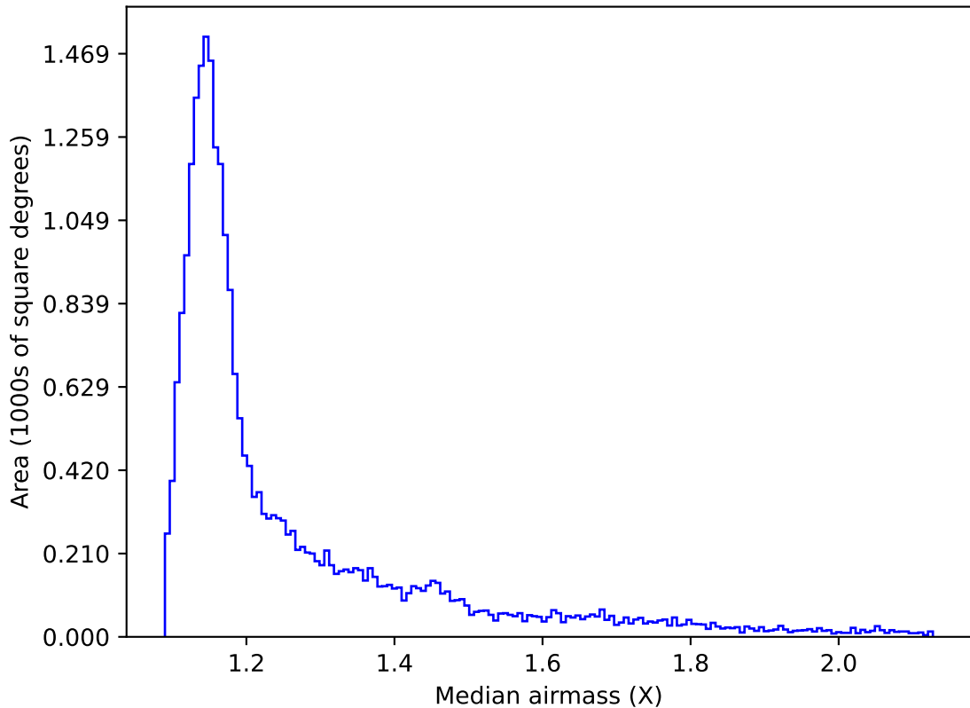
too_elab_r16_d3_griz_v3.4_10yrs All sky z band: Median airmass
