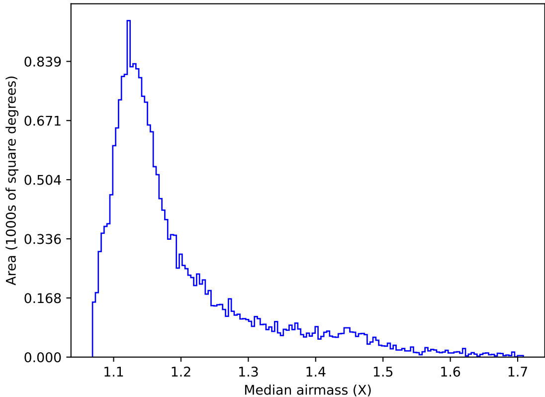
too_elab_r16_d3_griz_v3.4_10yrs All sky u band: Median airmass
