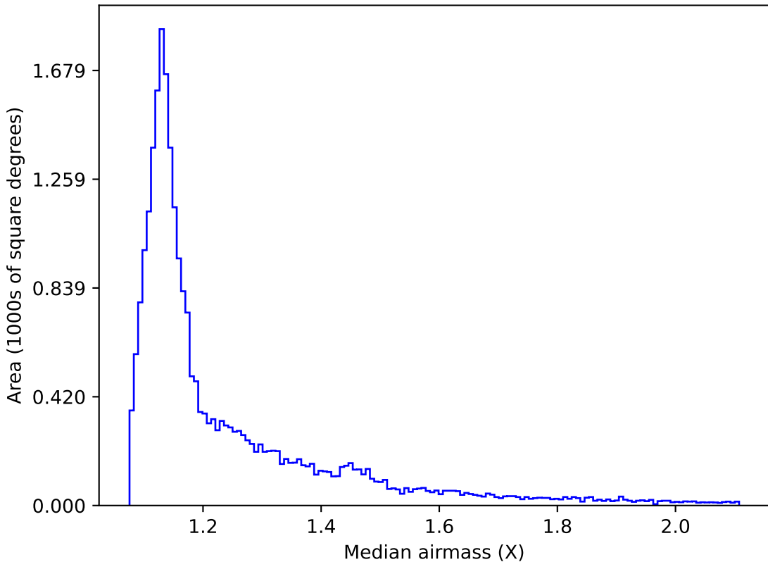
too_elab_r16_d3_griz_v3.4_10yrs All sky r band: Median airmass
