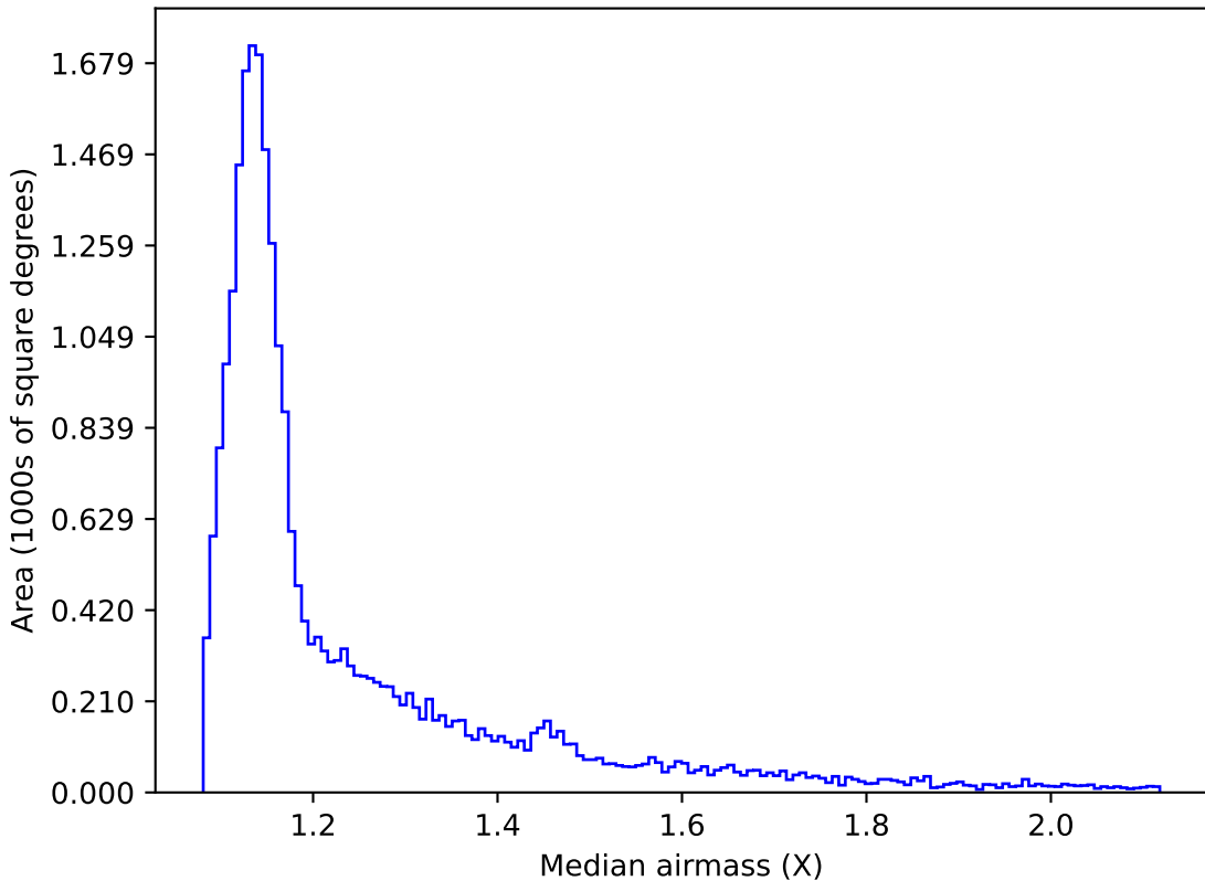
too_elab_r16_d3_griz_v3.4_10yrs All sky i band: Median airmass
