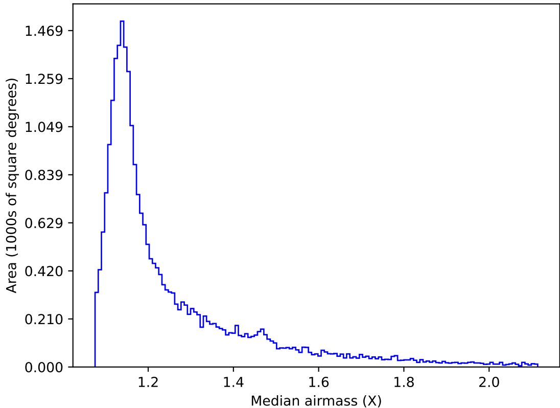
too_elab_r16_d3_griz_v3.4_10yrs All sky g band: Median airmass
