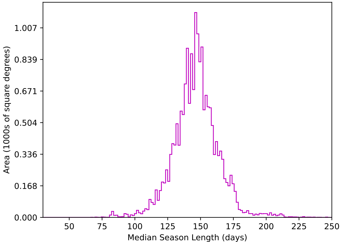
too_elab_r16_d3_griz_v3.4_10yrs WFD z band: Median Season Length
