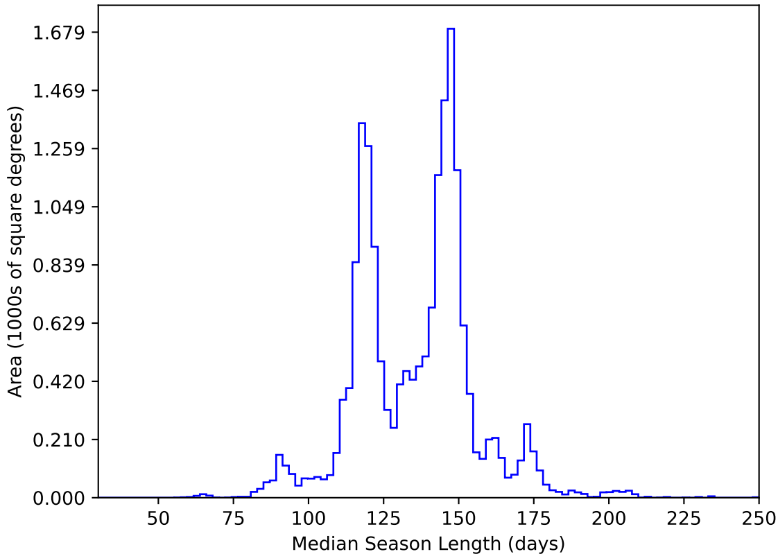
too_elab_r16_d3_griz_v3.4_10yrs WFD y band: Median Season Length
