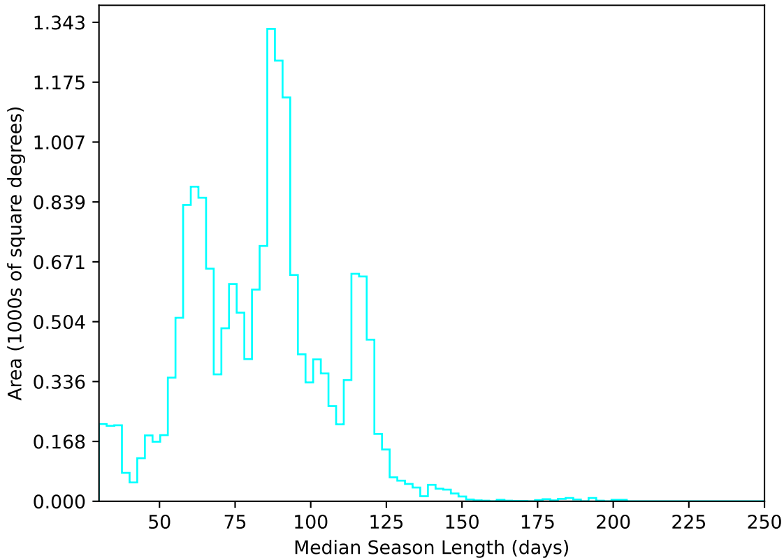
too_elab_r16_d3_griz_v3.4_10yrs WFD u band: Median Season Length
