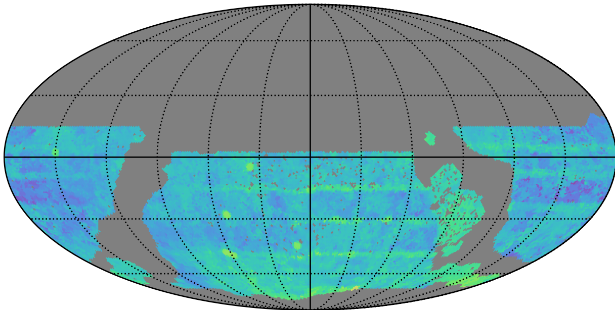
too_elab_r16_d3_griz_v3.4_10yrs WFD r band: Median Season Length
