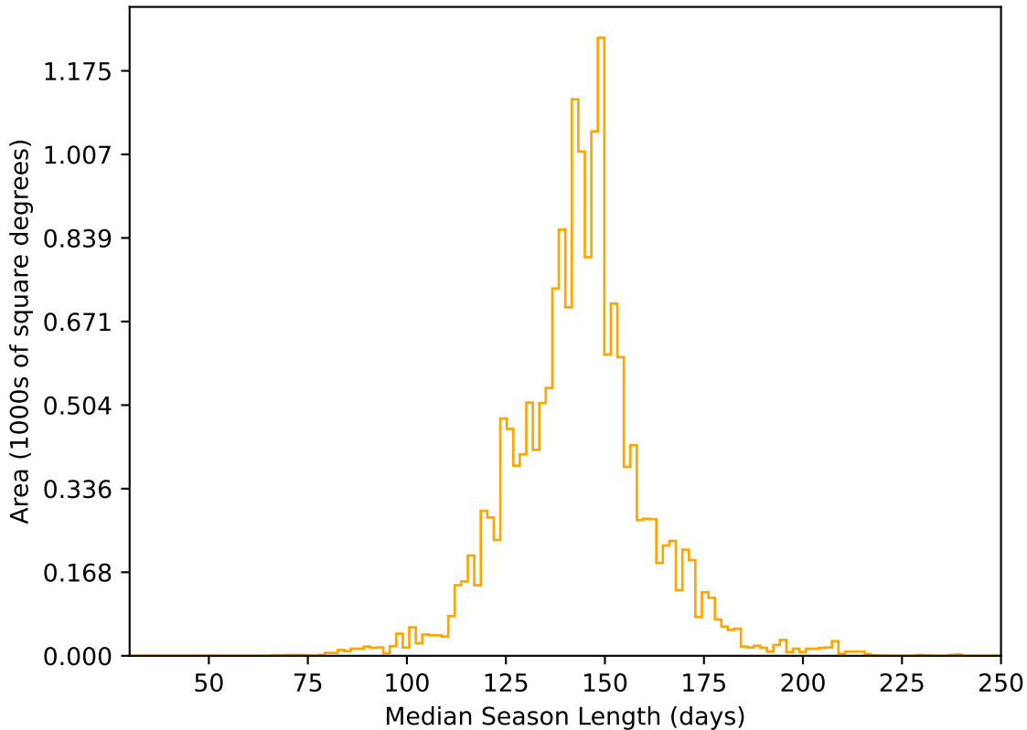
too_elab_r16_d3_griz_v3.4_10yrs WFD r band: Median Season Length
