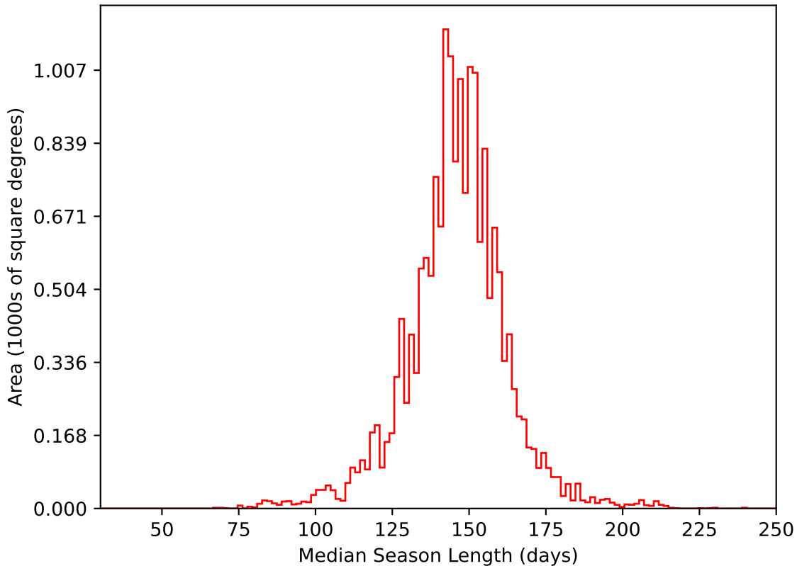
too_elab_r16_d3_griz_v3.4_10yrs WFD i band: Median Season Length
