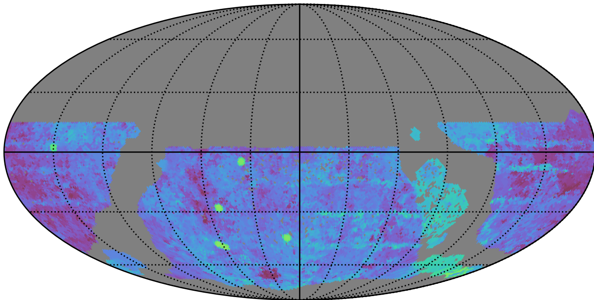
too_elab_r16_d3_griz_v3.4_10yrs WFD g band: Median Season Length
