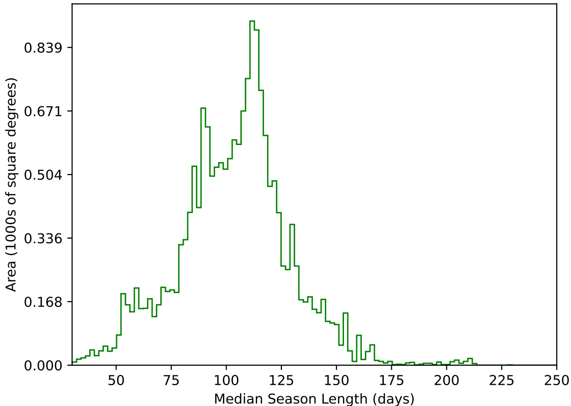
too_elab_r16_d3_griz_v3.4_10yrs WFD g band: Median Season Length
