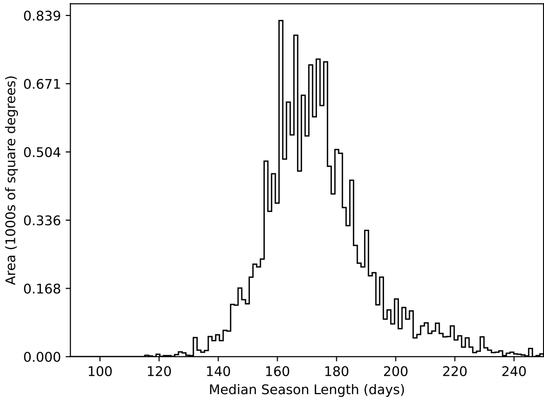
too_elab_r16_d3_griz_v3.4_10yrs WFD all bands: Median Season Length
