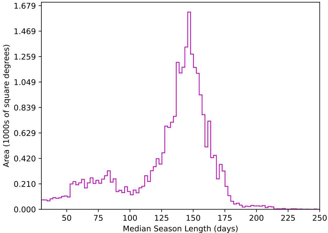
too_elab_r16_d3_griz_v3.4_10yrs All sky z band: Median Season Length
