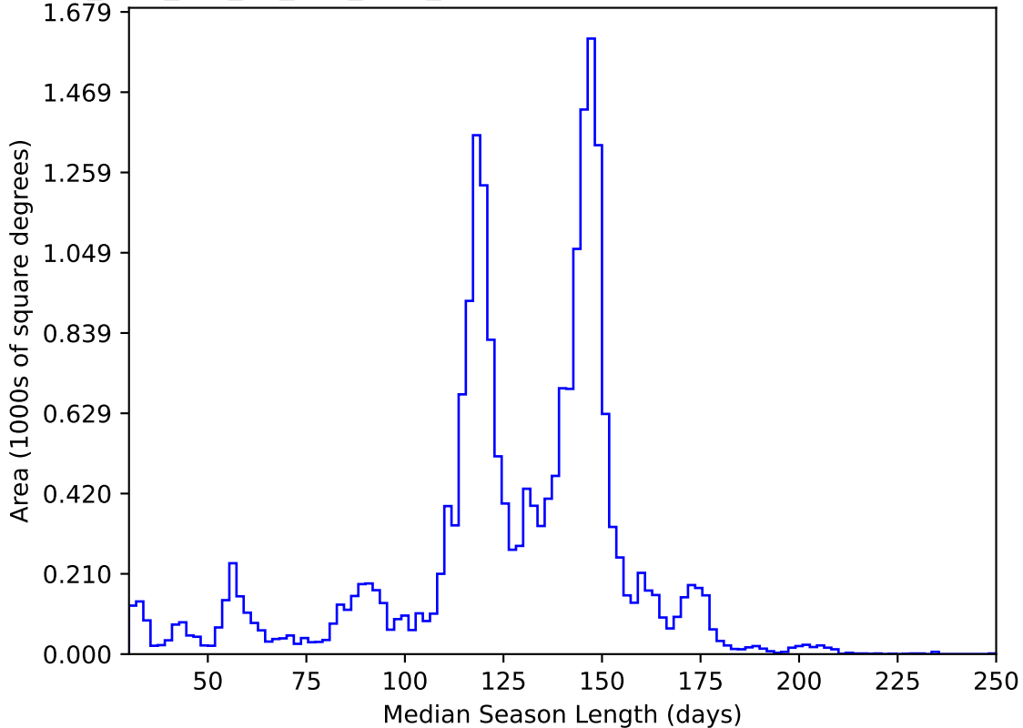
too_elab_r16_d3_griz_v3.4_10yrs All sky y band: Median Season Length
