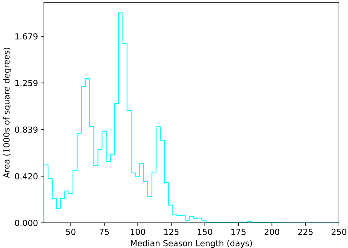
too_elab_r16_d3_griz_v3.4_10yrs All sky u band: Median Season Length
