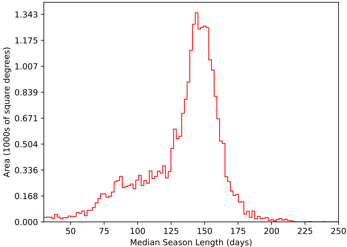
too_elab_r16_d3_griz_v3.4_10yrs All sky i band: Median Season Length
