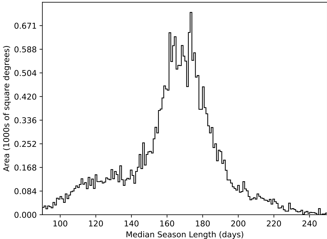
too_elab_r16_d3_griz_v3.4_10yrs All sky all bands: Median Season Length
