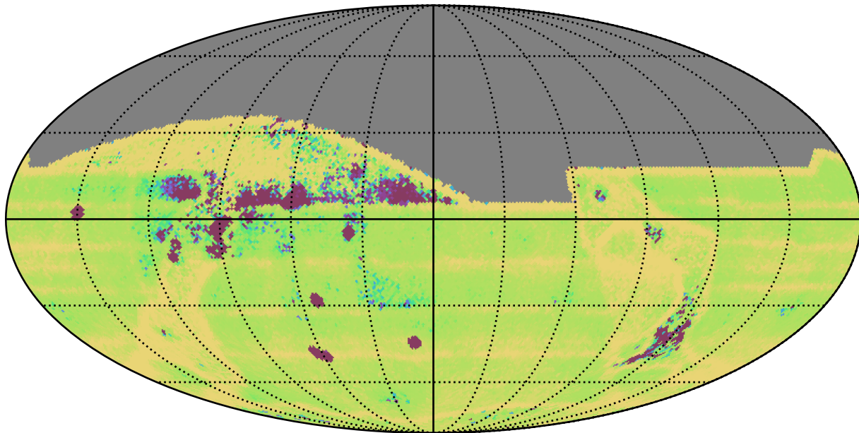
too_elab_r16_d3_griz_v3.4_10yrs All sky: Median Intra-Night Gap
